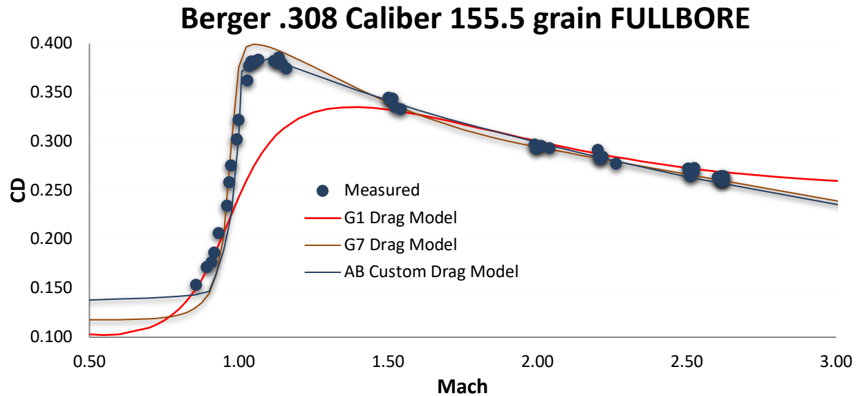
Figure 6. Custom Drag Model compared to the G1 and G7 standard curves.
