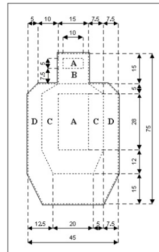
Figure 1. IPSC target. Dimensions in cm.
