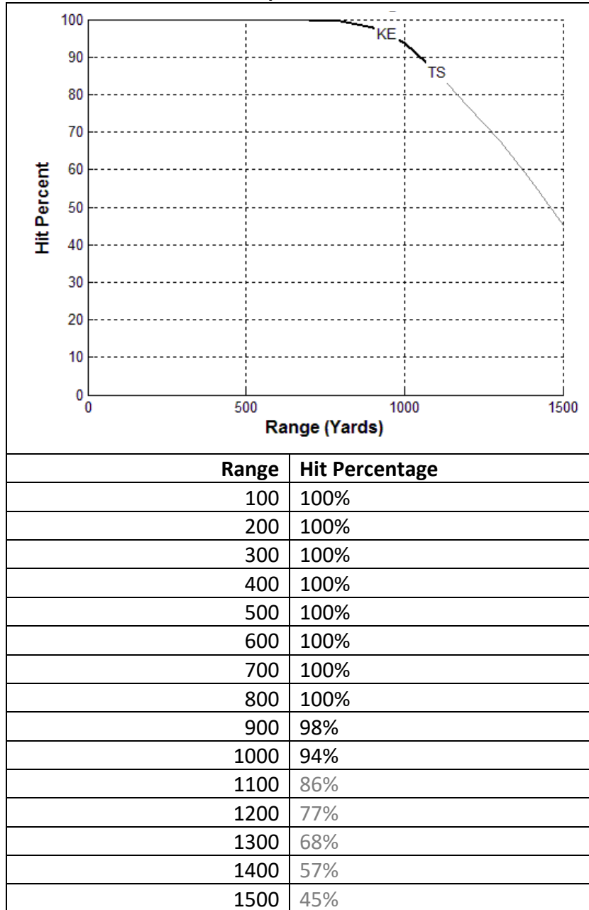
Figure 3. This plot and table shows the hit percentage as a function of range. This is the same information gathered by the method illustrated in Figure 2, but in a more analytical
